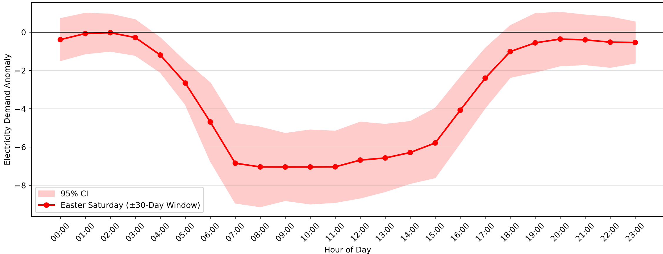
Homebush Bay Demand Anomaly: Easter Saturday (2004-2017, \pm 30 -Day Window)
